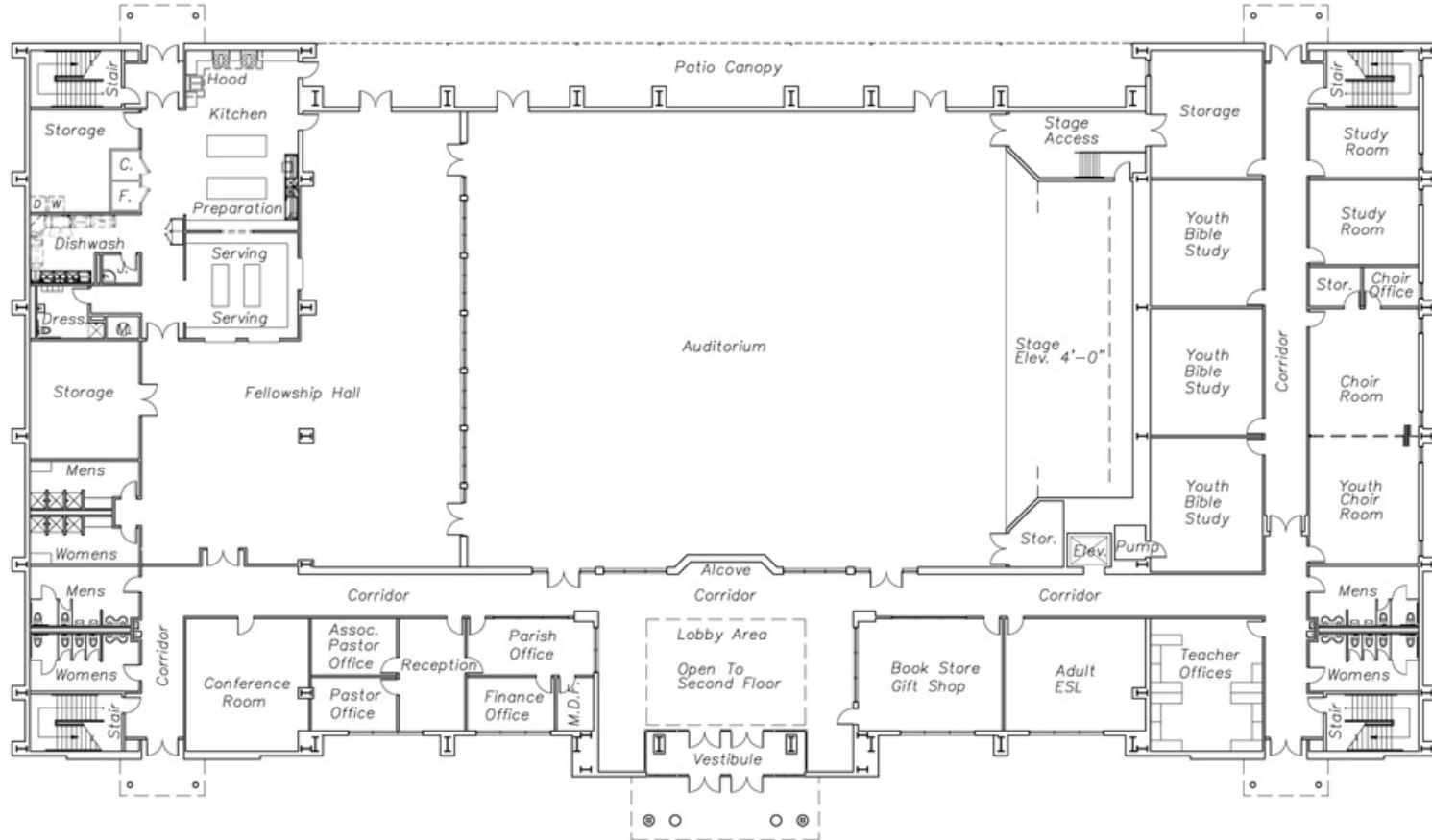
01 FIRST FLOOR PLAN SCALE 3/32" = 1'-0" NORTH
